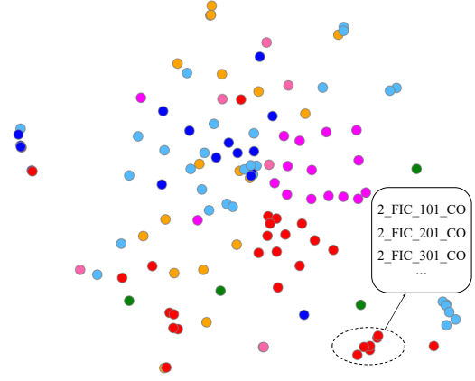
Figure 2: A t-SNE plot of the sensor embeddings of our trained model on the WADI dataset. Node colors denote classes. Specifically, the dashed circled region shows localized clustering of 2_FIC_x01_CO sensors. These sensors are measuring similar indicators in WADI.
